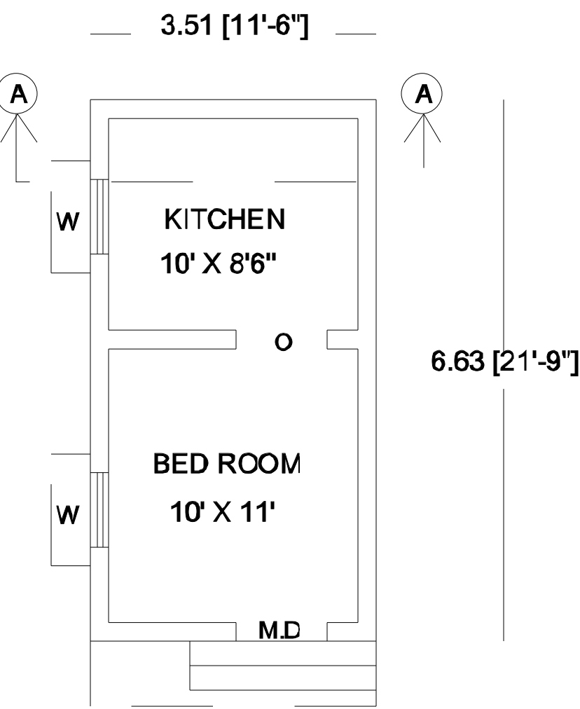
PLAN
