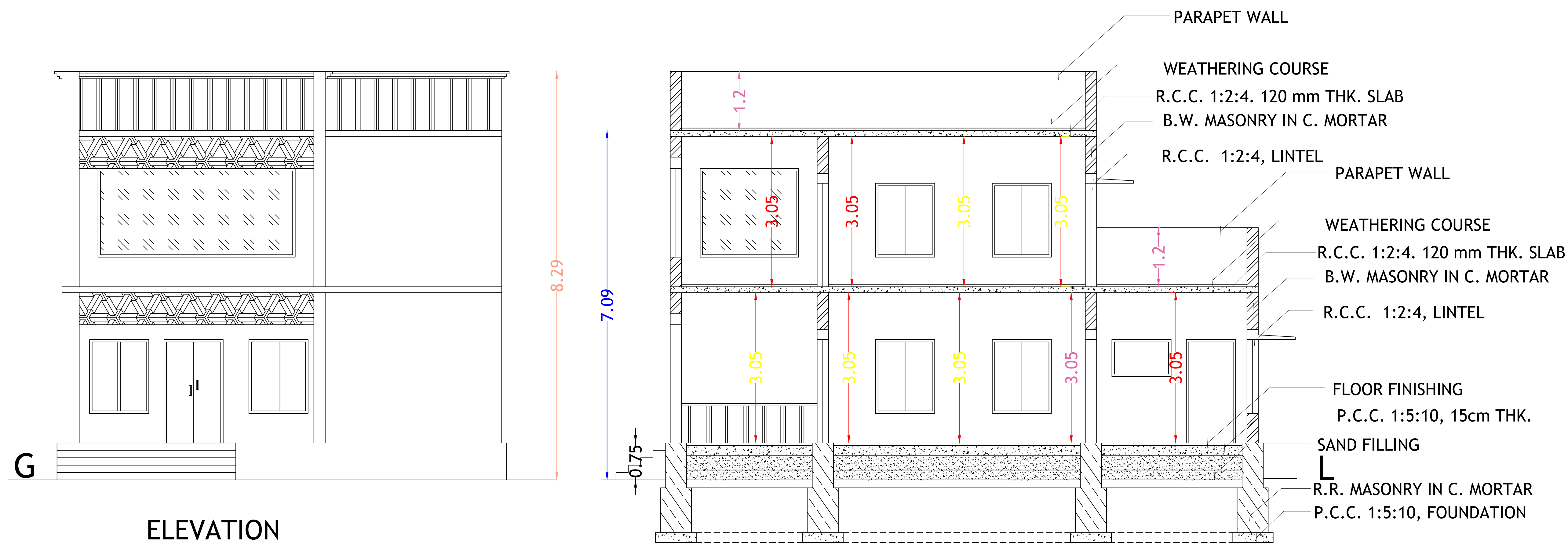
SECTION ON A-B
