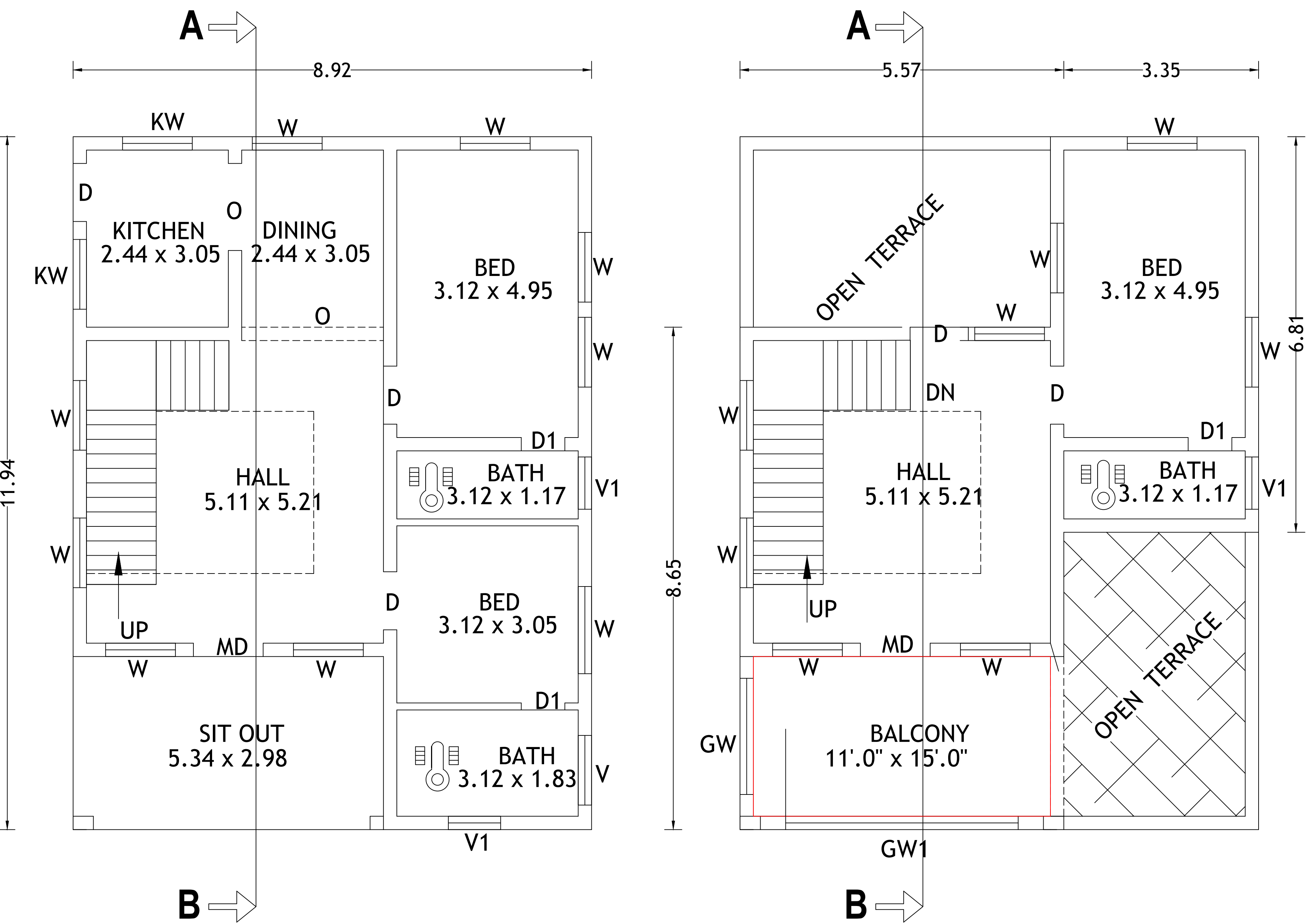
PLAN GROUND FLOOR
