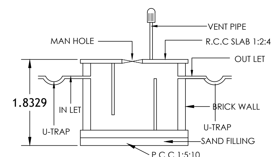
SECTION E,F SEPTIC TANK DETAIL
