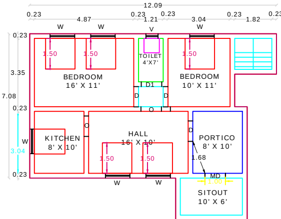
GROUND FLOOR RESIDENTIAL PLAN
