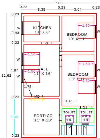
GROUND FLOOR RESIDENTIAL PLAN
