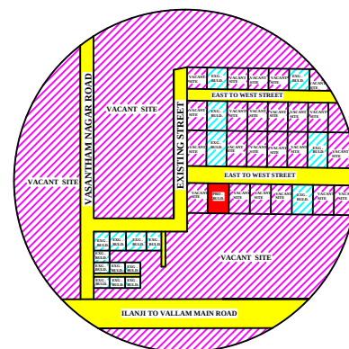
TOPO PLAN
