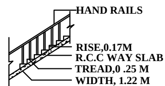
SECTION ON STAIR
