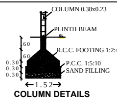
COLUMN DETAILS
