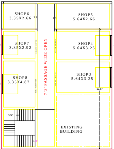
PRO FIRST FLOOR COMMERCIAL PLAN
