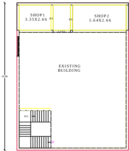
PRO GROUND FLOOR COMMERCIAL PLAN
