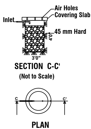
RainWater Perculation Pit (Not to Scale)
