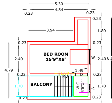
PRO FIRST FLOOR RESIDENTIAL PLAN
