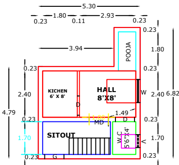
PRO GROUND FLOOR RESIDENTIAL PLAN
