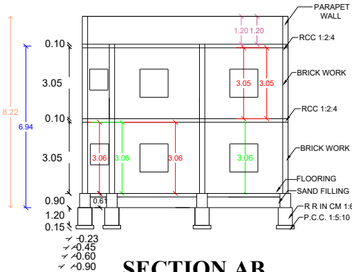
SECTION AB
