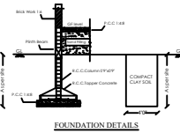
FOUNDATION DETAILS
