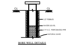
BORE WELL DETAILS
