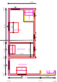
GROUND FLOOR PLAN (PROPOSED)
