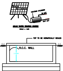
RWH SECTION (SAMPLE)
