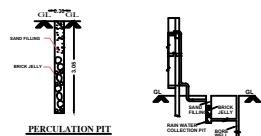
PERCOLATION PIT
