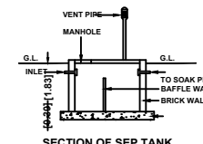
SECTION OF SEPTIC TANK
