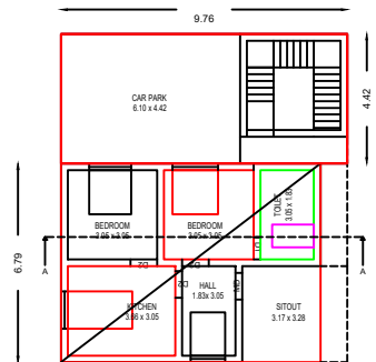
EXI / PRO GROUND FLOOR PLAN
