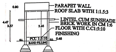
SECTION ON "AA"
