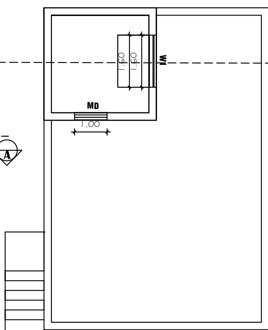
FIRST FLOOR PLAN (PROPOSED)
