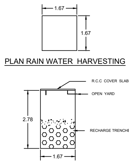
SECTION OF RAINWATER COLLECTING TANK
