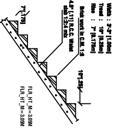
Staircase details (Not to scale)
