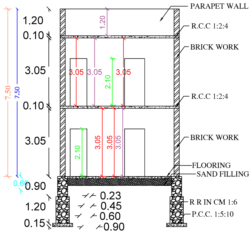
SECTION AB
