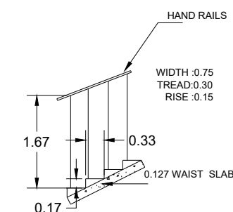
STAIRCASE DETAILS
