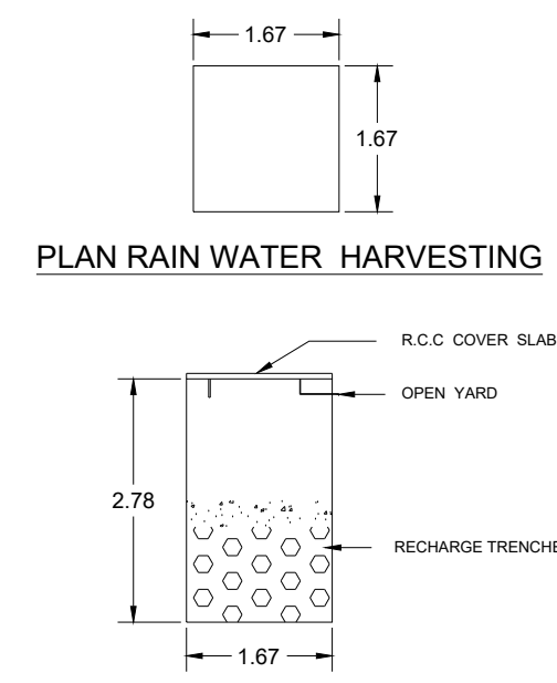
SECTION OF RAINWATER COLLECTING TANK
