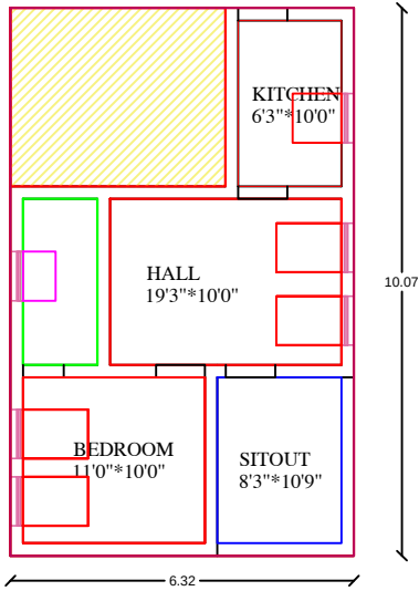
PROPOSED G.FLOOR PLAN
