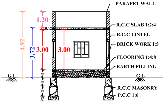
"SECTION "AB"
