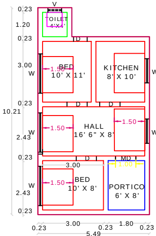
GROUND FLOOR RESIDENTIAL PLAN
