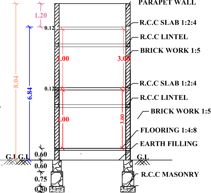
"SECTION 'AB'"
