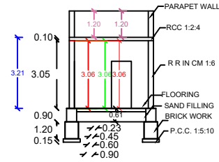
SECTION AB
