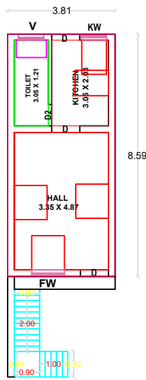
PLAN - GROUND FLOOR (PROPOSED)
