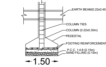
FOUNDATION DETAILS
