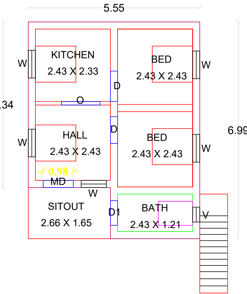
PLAN
