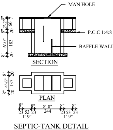
SEPTIC-TANK DETAIL
