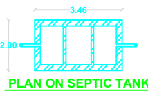
PLAN ON SEPTIC TANK
