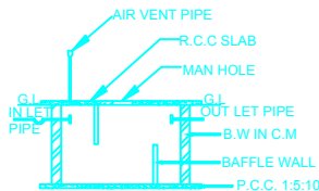
SECTION ON SEPTIC TANK
