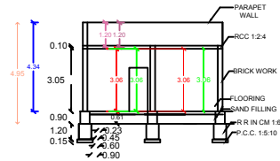
SECTION AB
