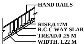
SECTION ON STAIR
