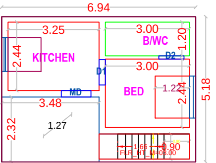
PLAN - FIRST FLOOR (PRO.BUILDING)
