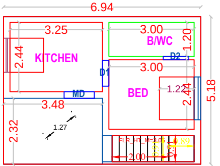
PLAN - GROUND FLOOR (PRO.BUILDING)
