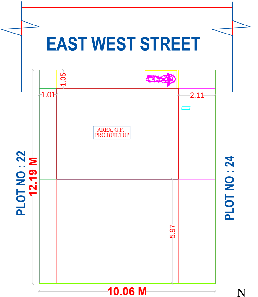
SURVRY NO : 560 SITE PLAN SCALE:- 1:100
