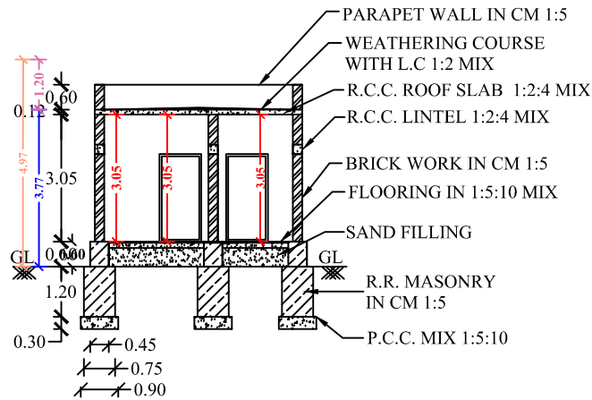
SECTION OF "AB"
