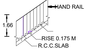
STAIRCASE
