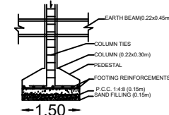
FOUNDATION DETAILS
