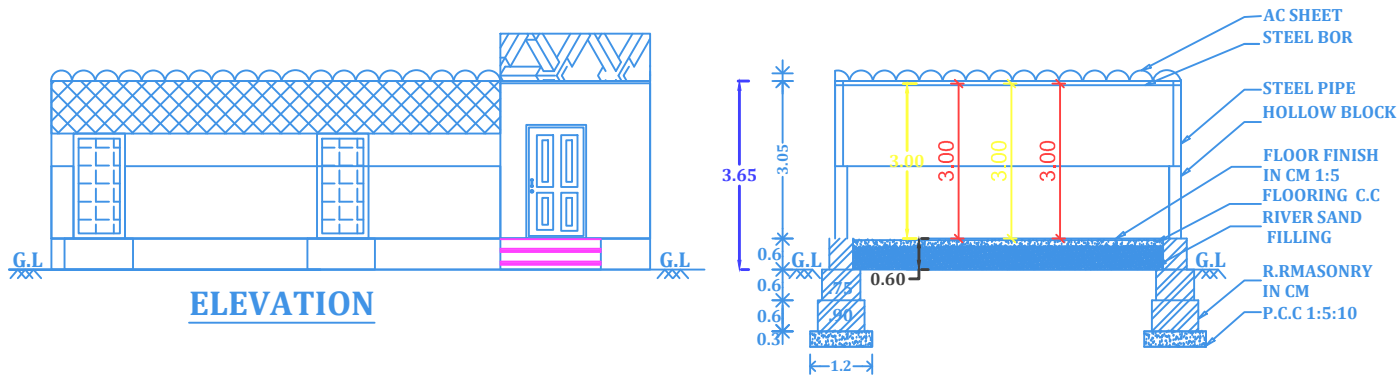
SECTION ON AA1
