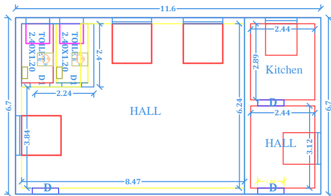
PLAN - GROUND FLOOR ( PROPOSED )
