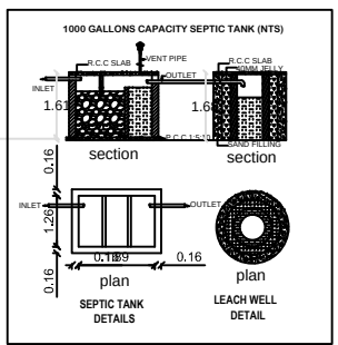
SECTION ON SV
