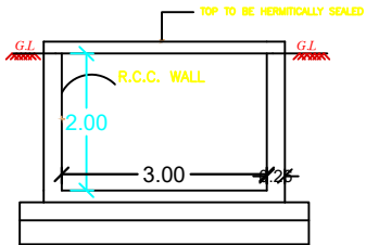
RWH SECTION
