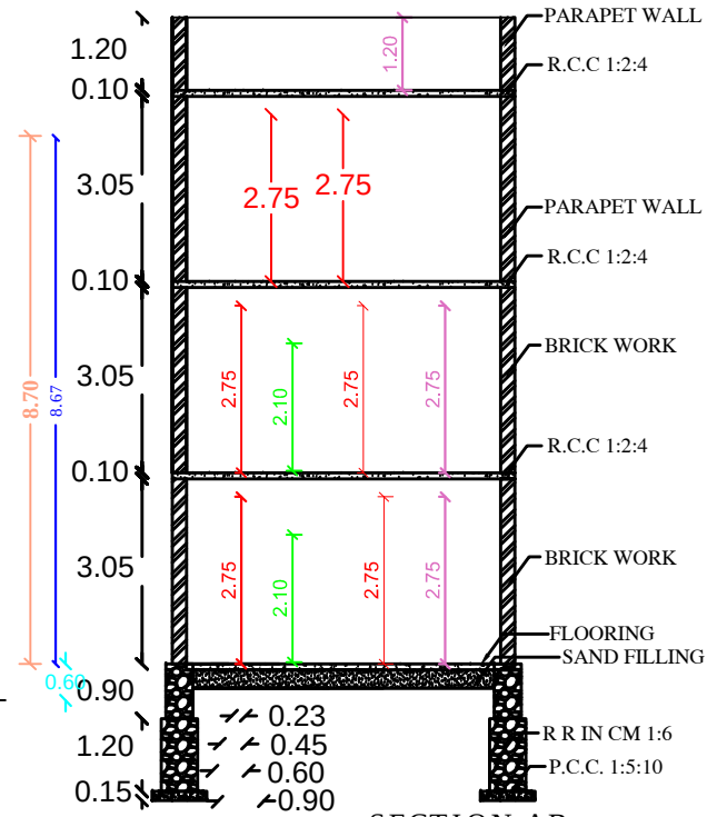
SECTION AB
