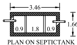
PLAN ON SEPTICTANK
