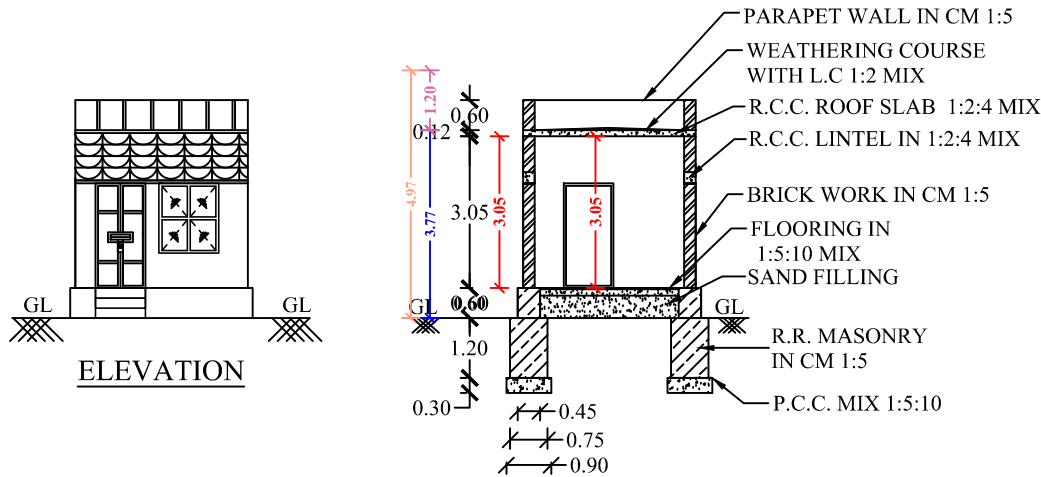
SECTION OF "AB"
