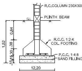
FOUNDATION DETAIL
