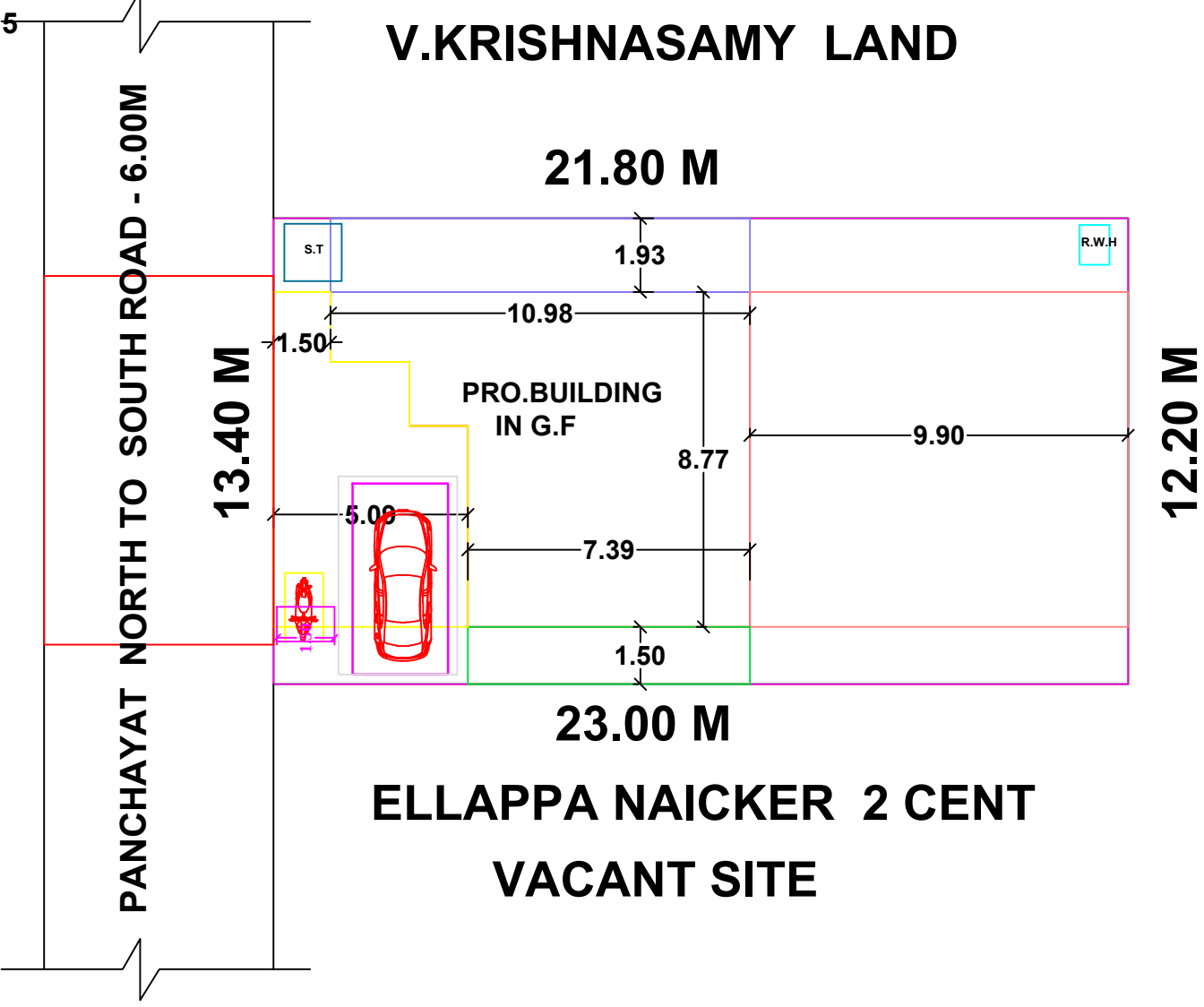
SITE PLAN
