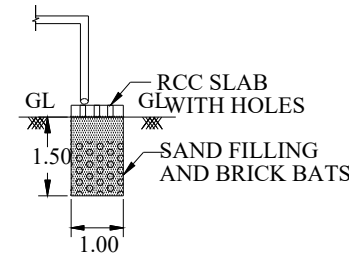
SECTION OF BS
