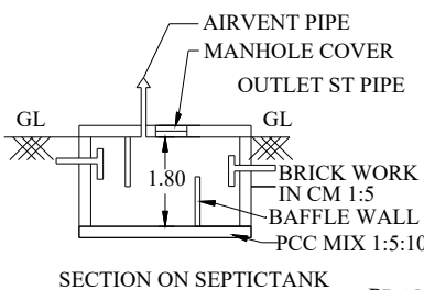
SECTION ON SEPTICTANK
