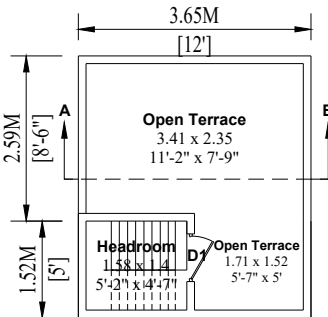
HEADROOM PLAN
