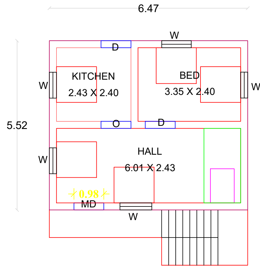
PLAN
