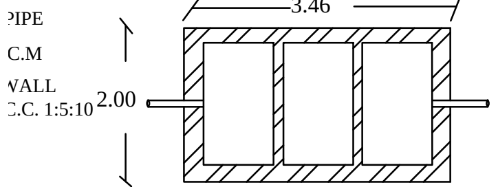
PLAN ON SEPTIC TANK
