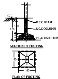
COLUMN DETAILS
