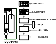
SOLAR SYSTEM
