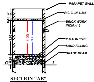
SECTION "AB"
