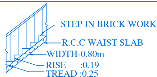
STAIR DETAIL
