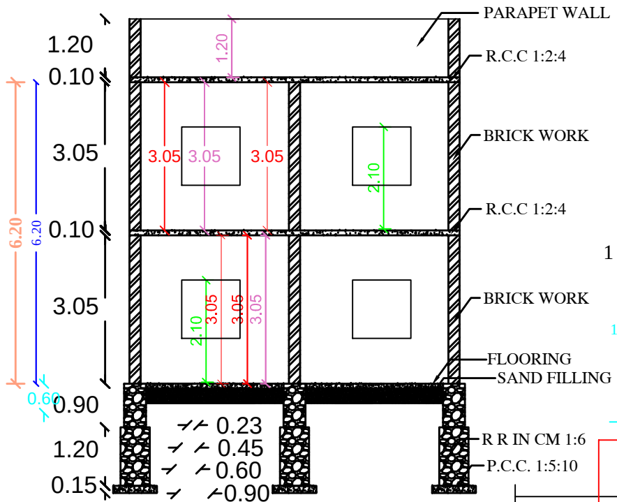
SECTION AB
