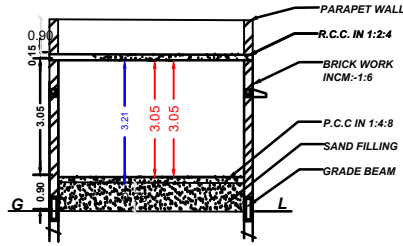
SECTION "AB"
