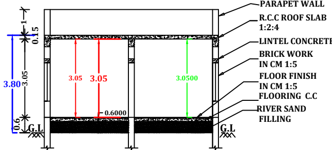
SECTION ON AA1
