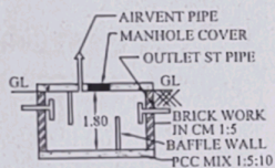
SECTION ON SEPTICTANK
