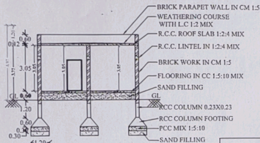
SECTION OF "AB"
