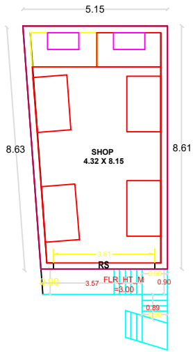
PLAN - GROUND FLOOR ( PROPOSED )
