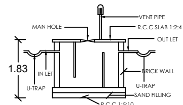
SECTION E-F SEPTIC TANK DETAIL
