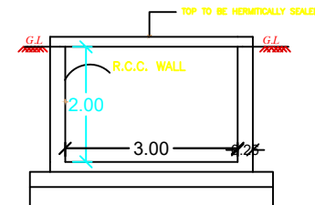
RWH SECTION
